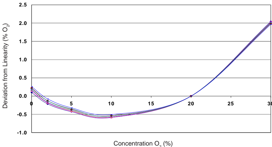
Figure 4 Linearity
