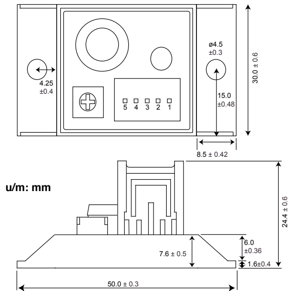
FCM6812 dimensions
