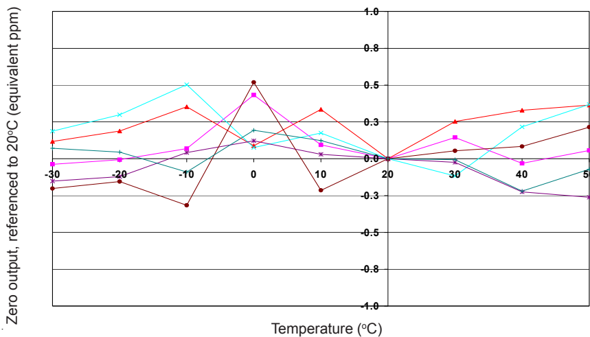
Figure 6 H 2 S Channel Zero Temperature Dependence
