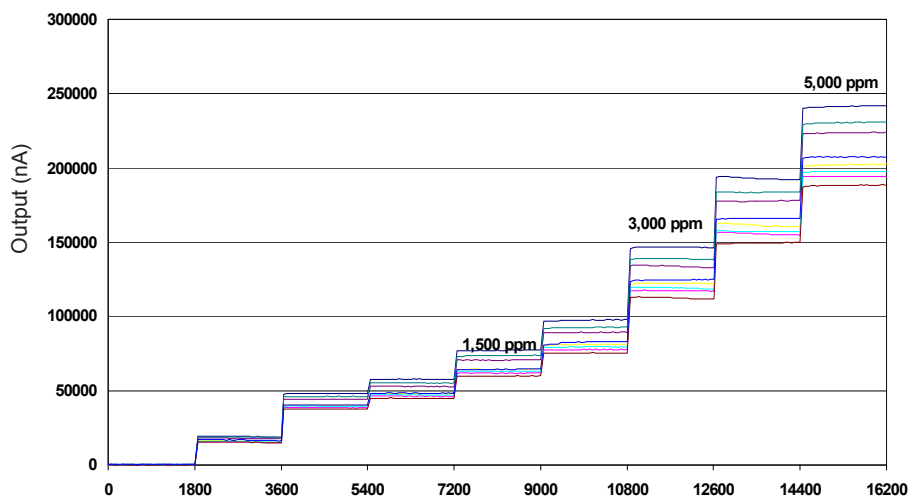
Figure 4 CO Channel Response to High CO Concentration
